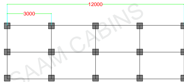
FOUNDATION PLAN PRECAST BLOCK SIZE 40 X 40 X 40
