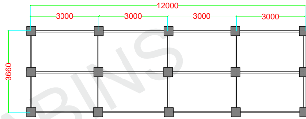
FOUNDATION PLAN PRECAST BLOCK SIZE 40 X 40 X 40
