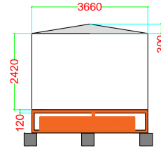
LEFT SIDE ELEVATION
