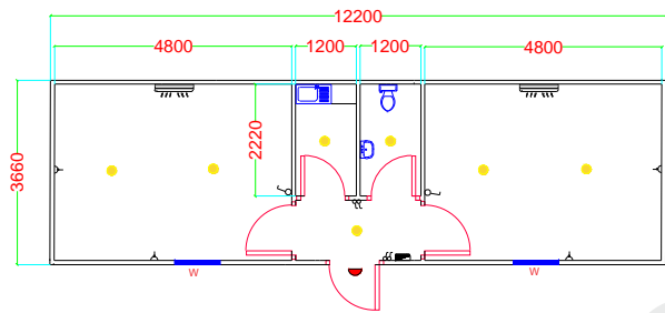
FLOOR PLAN
